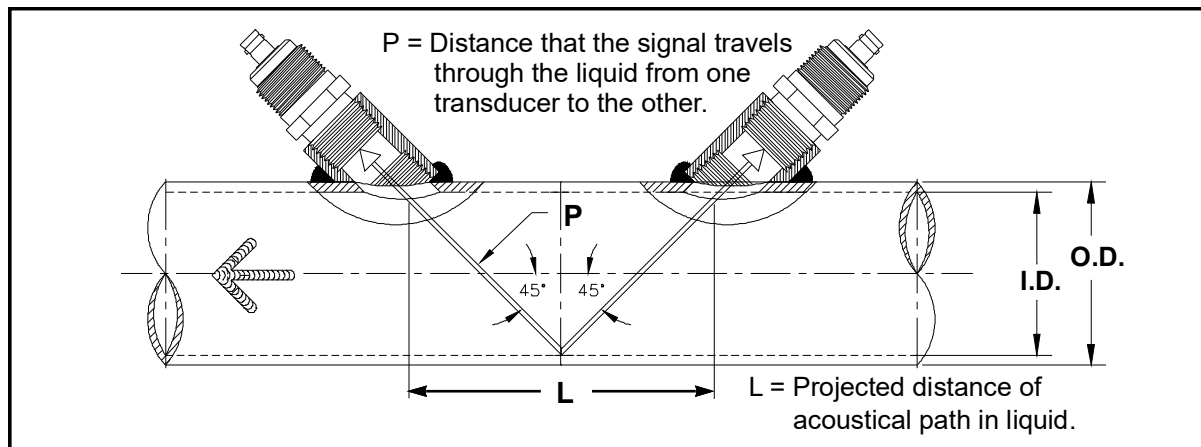
Figure 3: Double-Traverse Flowcell
