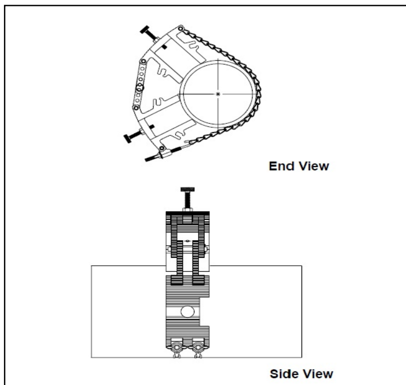
Figure 44: Completed <180^\circ Installation without Transducers
