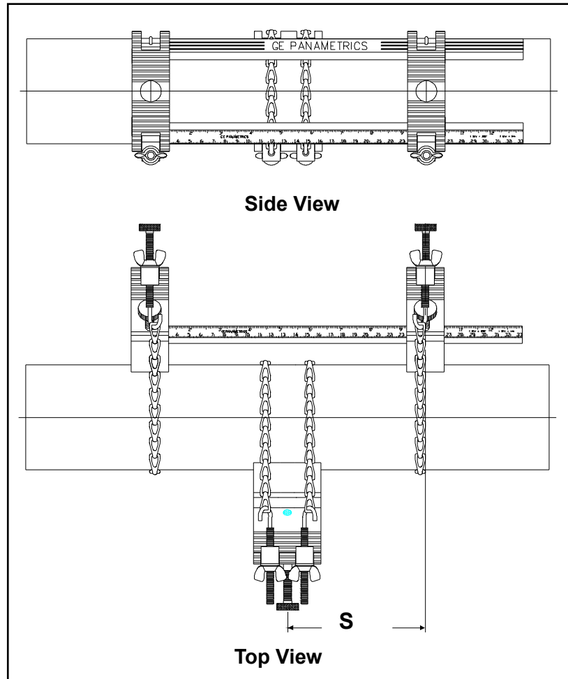
Figure 28: A Single-Traverse Clamping Fixture Installation without Transducers
