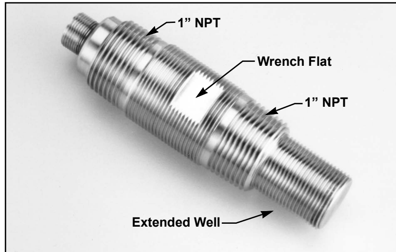
Figure 13: Extended-Well Transducer
