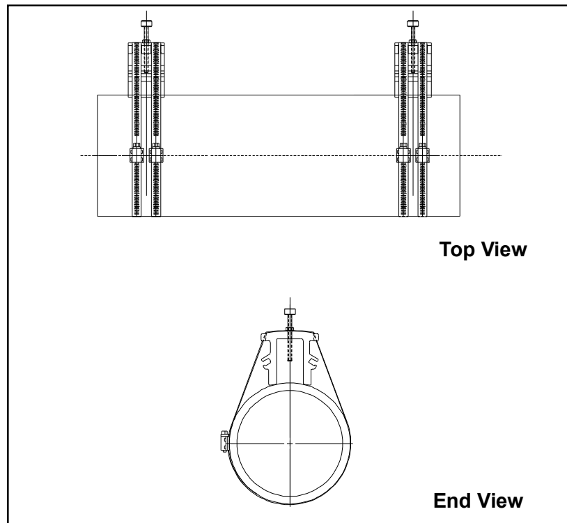
Figure 32: A Double-Traversal GCF Installation without Transducers
