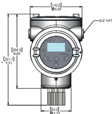
*8.96 [227.6] WEATHERPROOF VERSION
