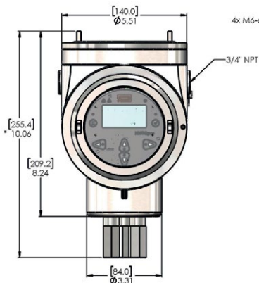
*9.11 [231.4] WEATHERPROOF VERSION
