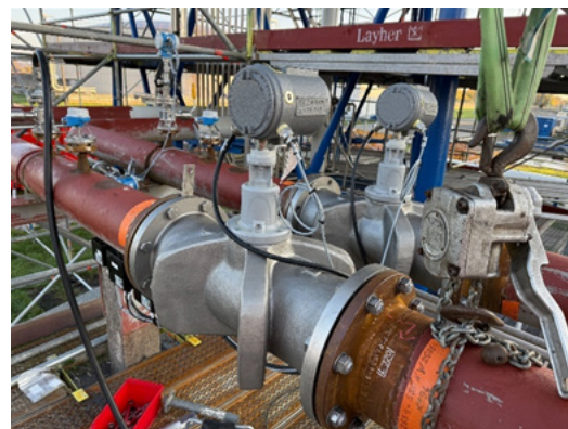
PanaFlow ZIG view from the back
