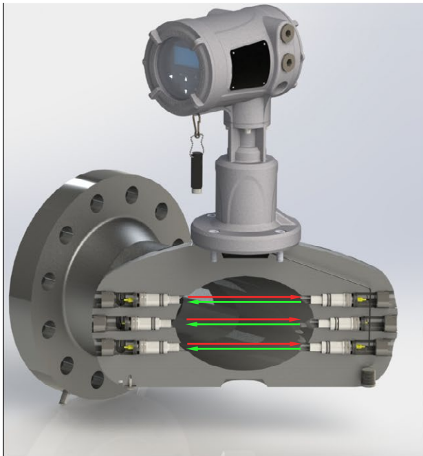
Transit time flow measurement
