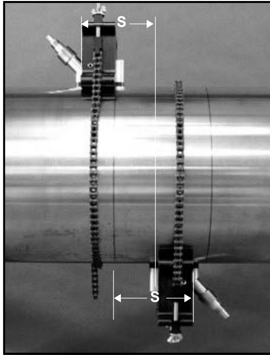
Figure 20: CFG-PI Fixture with Calculated Spacing
