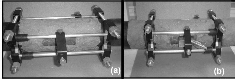
Figure 31: Clearing DMP-3 (a) and Installing Transducers (b)
