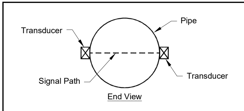
Figure 2: Desired Projection of Acoustical Signal Path
