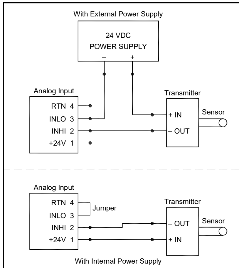
Figure 39: Analog Input Wiring Diagram
