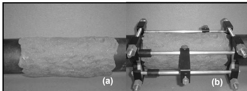
Figure 30: Spreading DMP-3 (a) and Reinstalling the Fixture (b)
