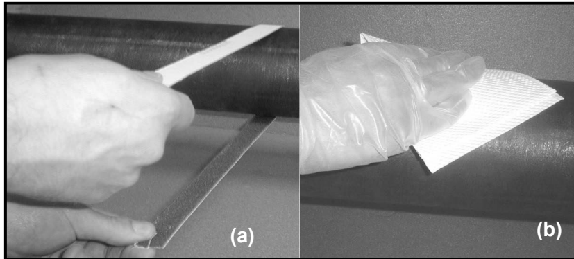
Figure 28: Filing (a) and Degreasing (b) the Pipe Surface
