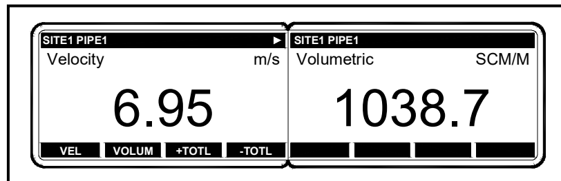
Figure 45: A Typical Measurement Display
