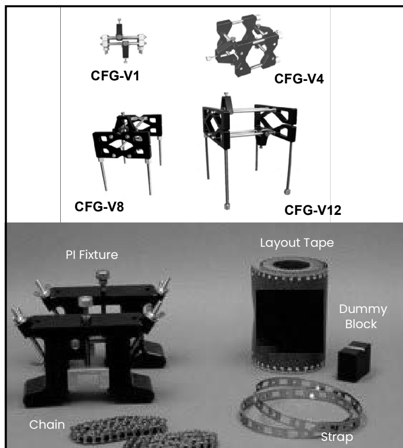
Figure 1: The V Series and PI Fixtures
