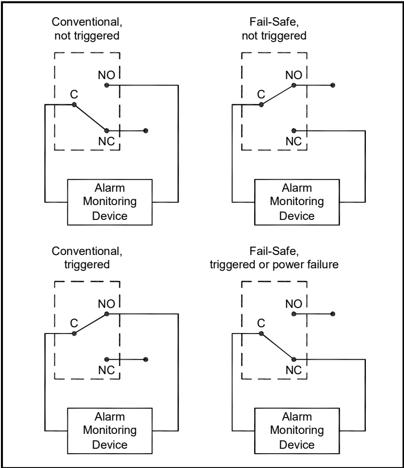
Figure 38: Conventional and Fail-Safe Operation
