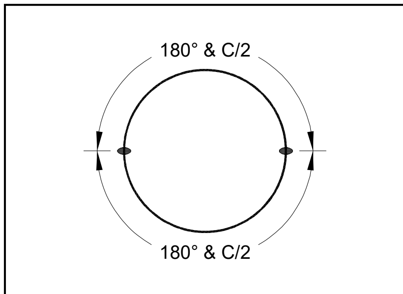
Figure 15: Measuring the 180° Point from Top and Bottom
