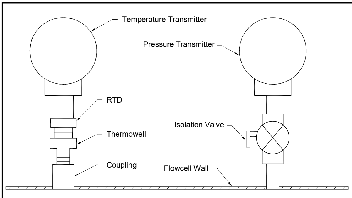
Figure 34: Typical Temperature/Pressure Transmitter Mounting
