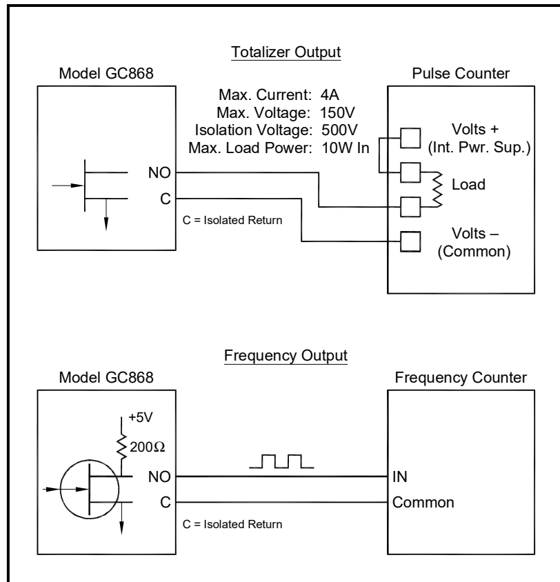
Figure 40: Totalizer/Frequency Outputs Wiring
