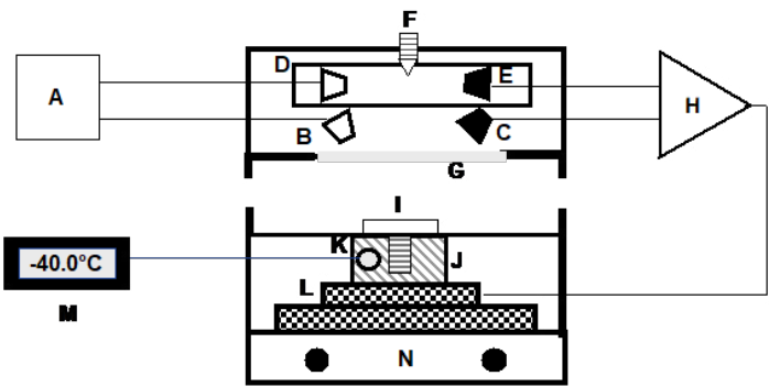
Figure 1. Automatic chilled mirror
