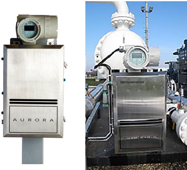
Figure 6. TDLAS hygrometer
