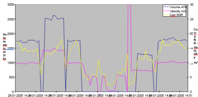
Flow rate measurement at Location 6
