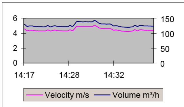
Flow rate measurement at Location 2
