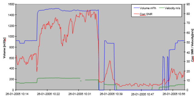
Flow rate measurement at Location 4 (Flow fluctuations shown above were caused by customer controlling the pressure downstream of the reducing valve.)
