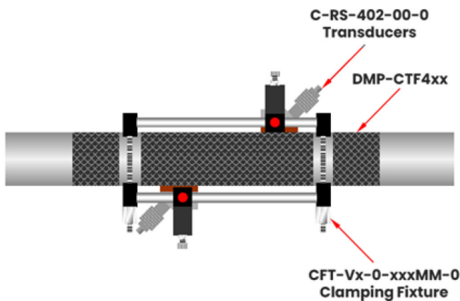
Triple-traverse installation
